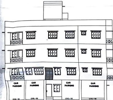
EAST SIDE ELEVATION SCALE: 1:100
